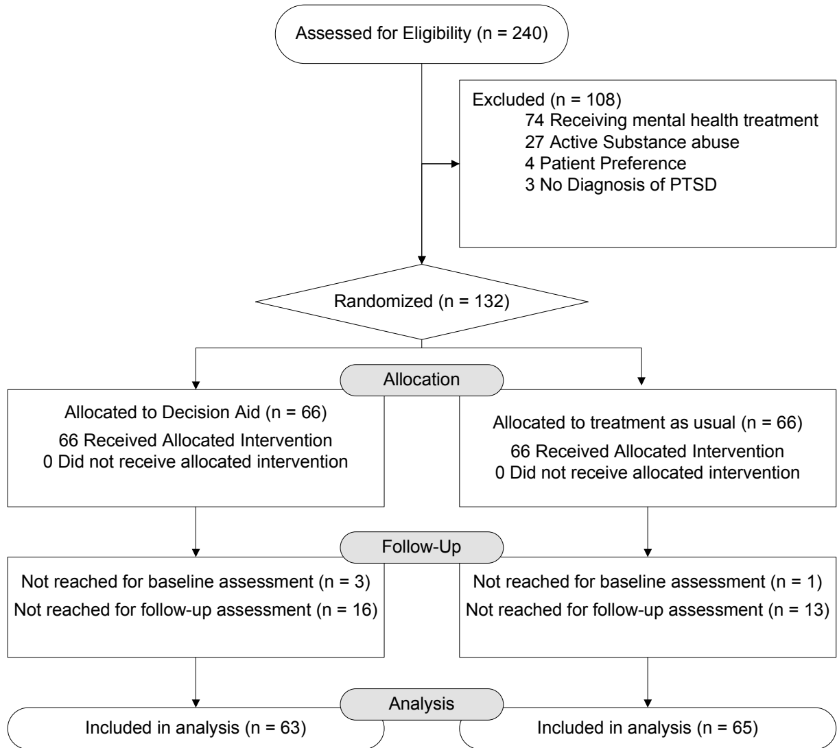
Figure 1: Consort Diagram
